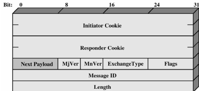
(a) ISAKMP Header
